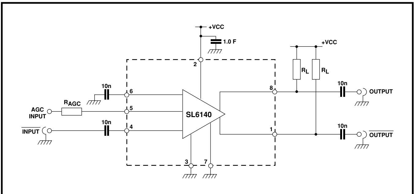
Figure 1 Typical Application
